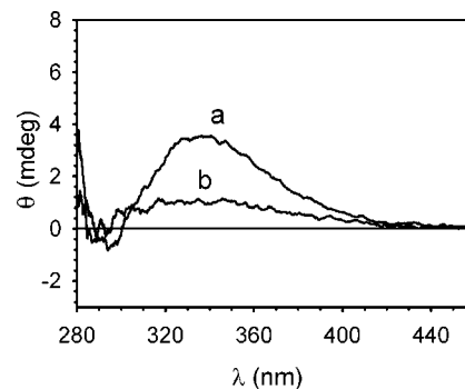
Figure 1. CD spectra at 309 K (cell path length 0.1 cm) of a 200 mM NaCl aqueous solution of 8.0 mM 1a in the presence of: (a) 40.0 mM surfactant 2a ; (b) 40.0 mM surfactant 2b .
